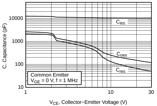
Figure 6. Capacitance Characteristics
