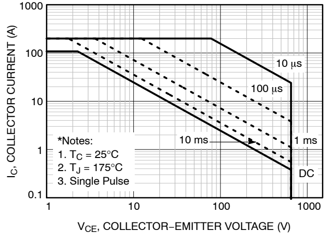
Figure 8. SOA Characteristics
