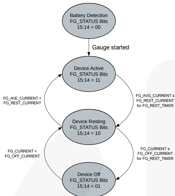
Figure 4. Gauging Modes
