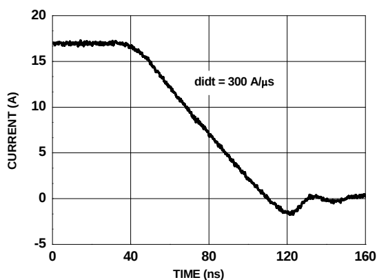
Figure 27. FDMS3668S SyncFET™ body diode reverse recovery characteristic
