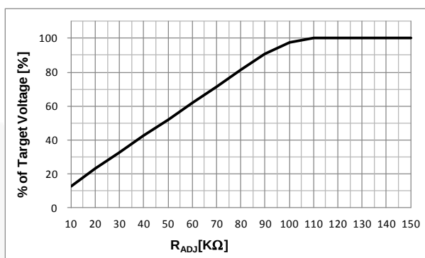
Figure 21. % of Sine Amplitude vs. R_{ADJ}
