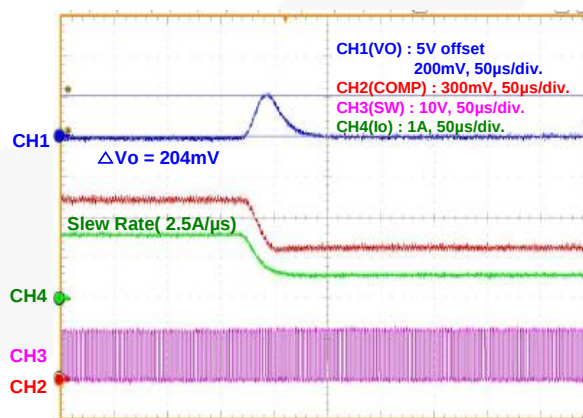
Figure 9. Load Transient Response (1.5 A to 0.5 A)
