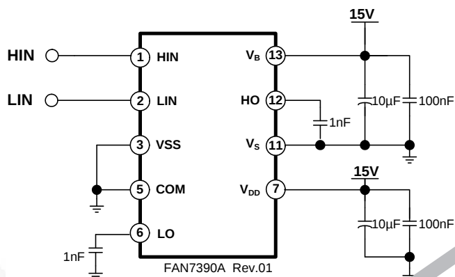
Figure 24. Switching Time Test Circuit (Reference 8-S)
