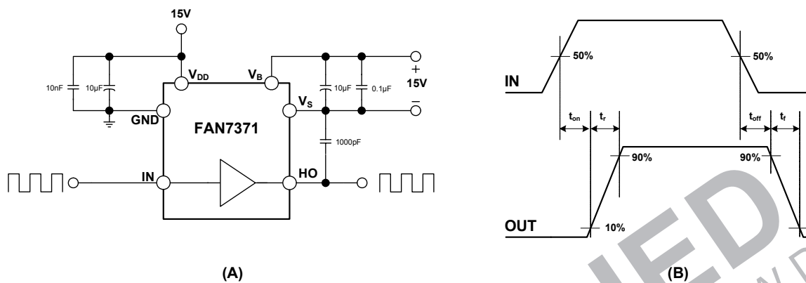
Figure 23. Switching Time Test Circuit and Waveform Definitions
