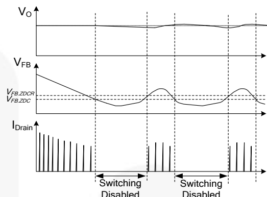
Figure 23. Burst Switching in Green Mode
