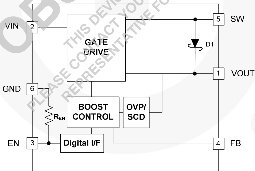
Figure 2. Block Diagram
