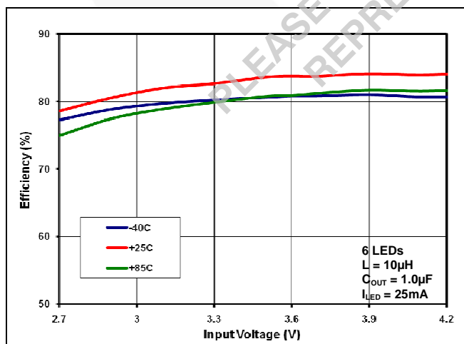
Figure 8. Efficiency vs. Input Voltage vs. Temperature
