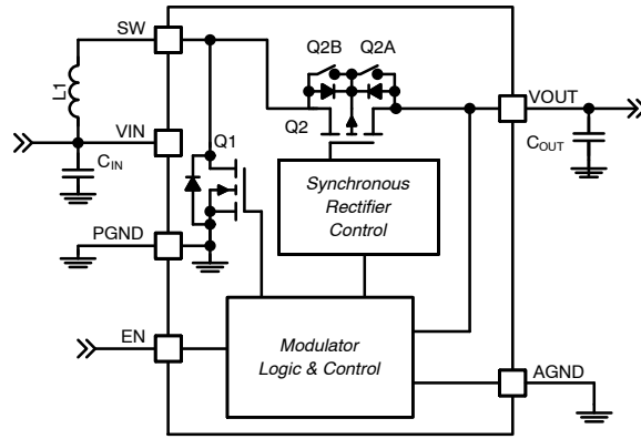
Figure 2. IC Block Diagram
