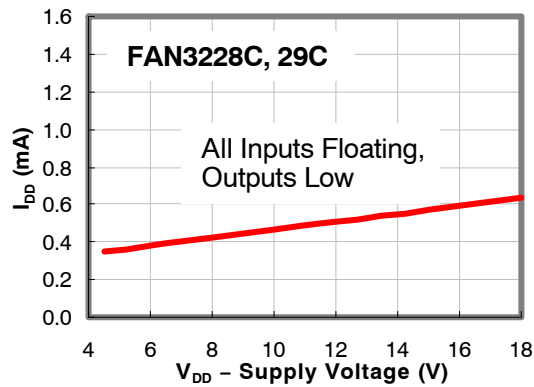
Figure 15. I_{DD} (Static) vs. Supply Voltage (Note 13)
