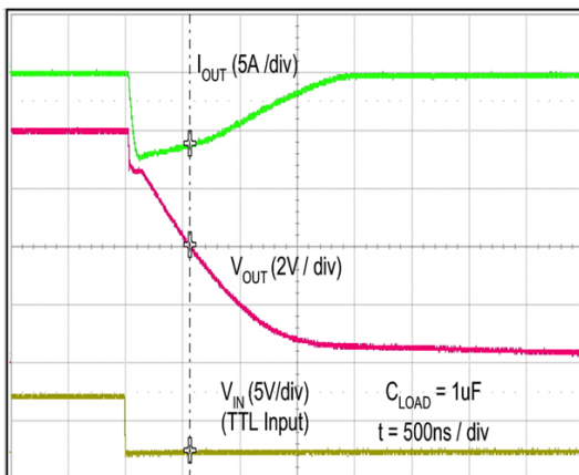
Figure 44. Quasi-Static Sink Current with VDD = 8 V (Note 14)
