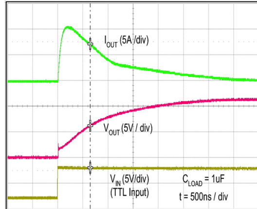
Figure 41. Quasi-Static Source Current with VDD = 12 V (Note 14)
