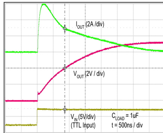
Figure 43. Quasi-Static Source Current with VDD = 8 V (Note 14)
