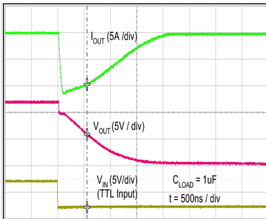
Figure 42. Quasi-Static Sink Current with VDD = 12 V (Note 14)
