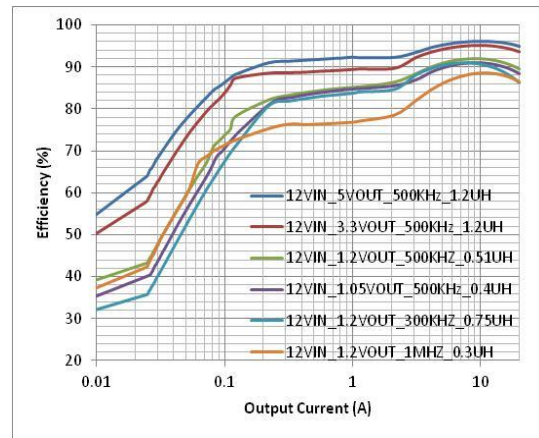
Figure 11. Efficiency vs. Load Current with V_{IN}=12\text{ V}
