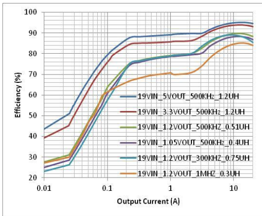
Figure 10. Efficiency vs. Load Current with V_{IN}=19\text{ V}
