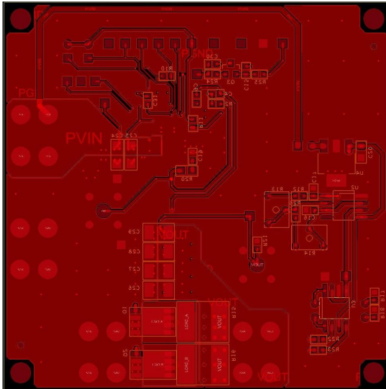
Figure 31. Evaluation Board Bottom Layer Copper
