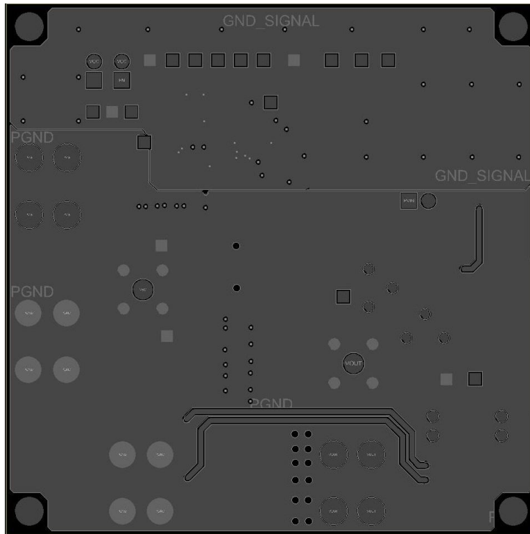
Figure 28. Evaluation Board Top Layer
