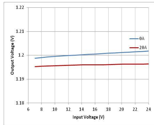
Figure 15. Line Regulation
