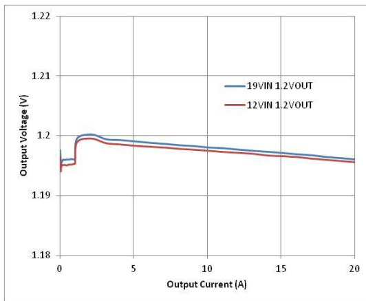
Figure 14. Load Regulation
