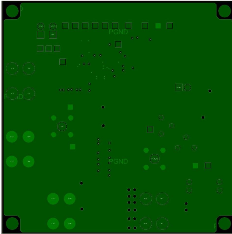
Figure 30. Evaluation Board Inner Layers 2,3, and 4 Copper
