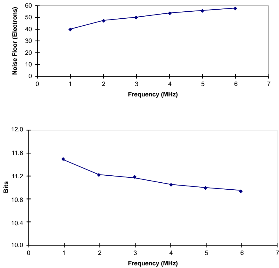
Figure 17. Measured Performance: Dynamic Range
