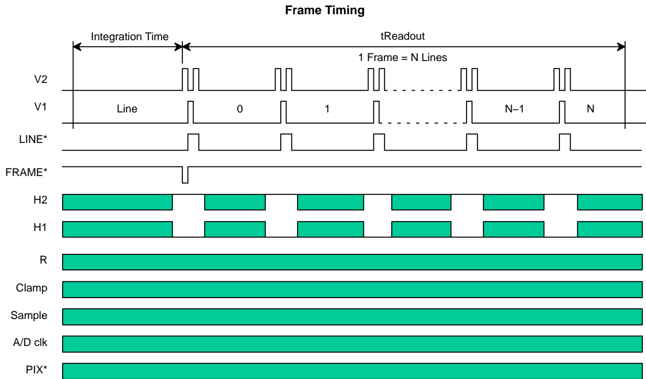
Figure 10. Frame Timing for the KAF-3200 Sensor
