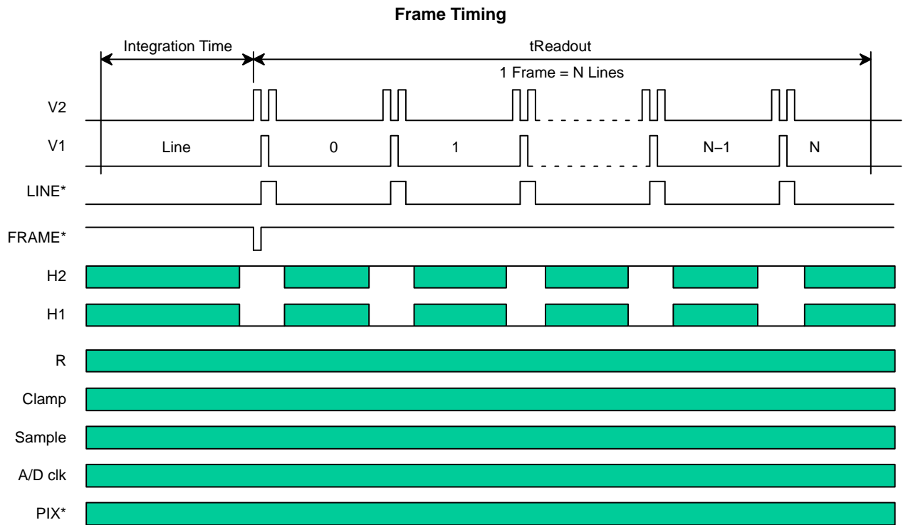
Figure 9. Frame Rate Timing for the KAF-0261, 0402, 1001, 1603, 4301, 6303, 16801
