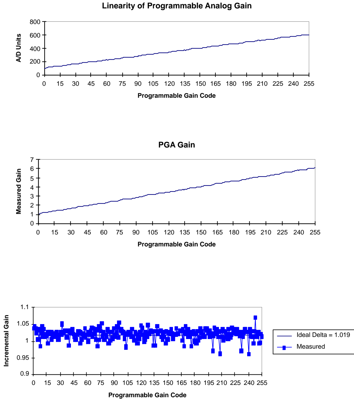
Figure 18. Measured Performance: A/D Programmable Gain
