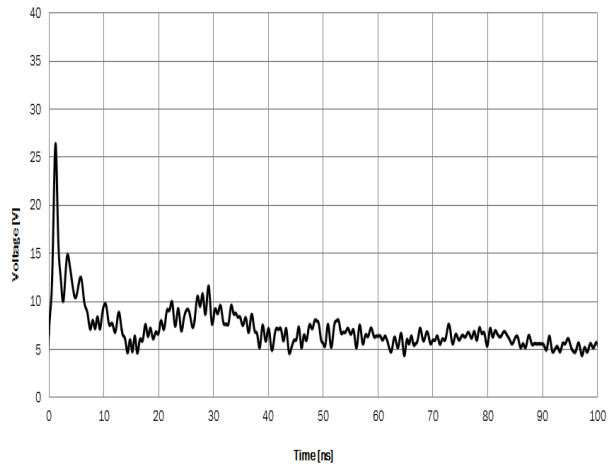
Figure 6. Positive 8 kV ESD Contact Discharge
