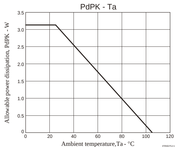
Allowable power dissipation, PdPK(no heat sink) - Ambient temperature, Ta
