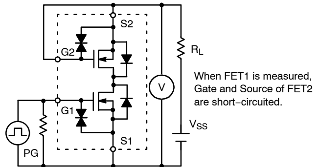
Figure 6. Test Circuit 6 - t_{d(on)} , t_r , t_{d(off)} , t_f
