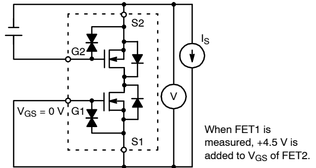
Figure 8. Test Circuit 8 - V_{F(s-s)}
