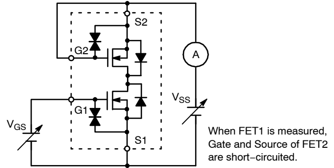
Figure 4. Test Circuit 4 - g_{FS}
