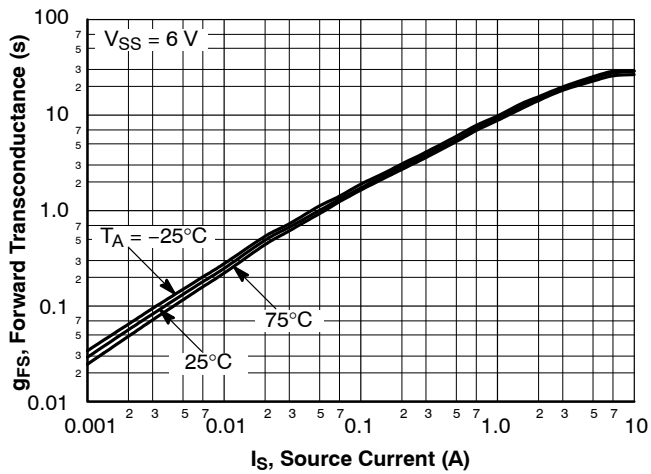
Figure 13. g_{FS} - I_S
