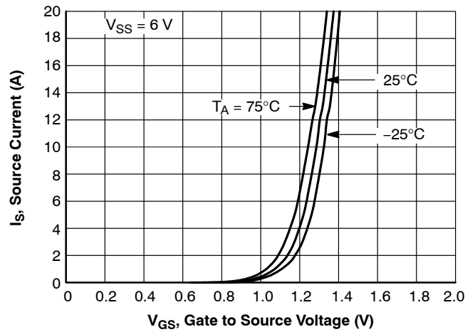
Figure 10. I_S - V_{GS(th)}
