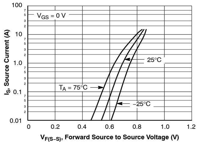
Figure 14. I_S - V_{F(S-S)}
