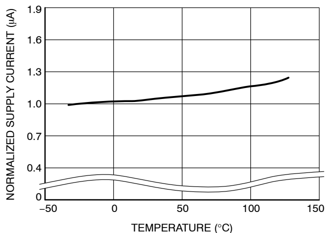
Figure 3. Supply Current vs. Temperature (No Load, CAX8xxR/S/T/Z)
