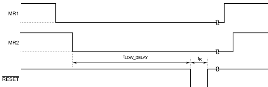
Figure 3. Timing Waveforms
