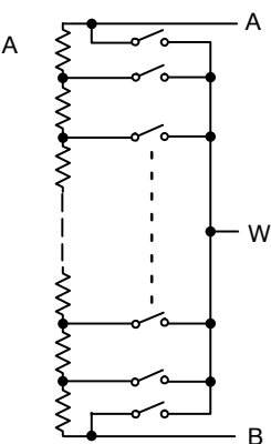
Figure 3. Electronic Potentiometer Implementation
