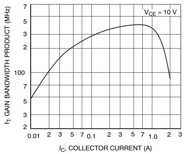
Figure 4. f_T - I_C
