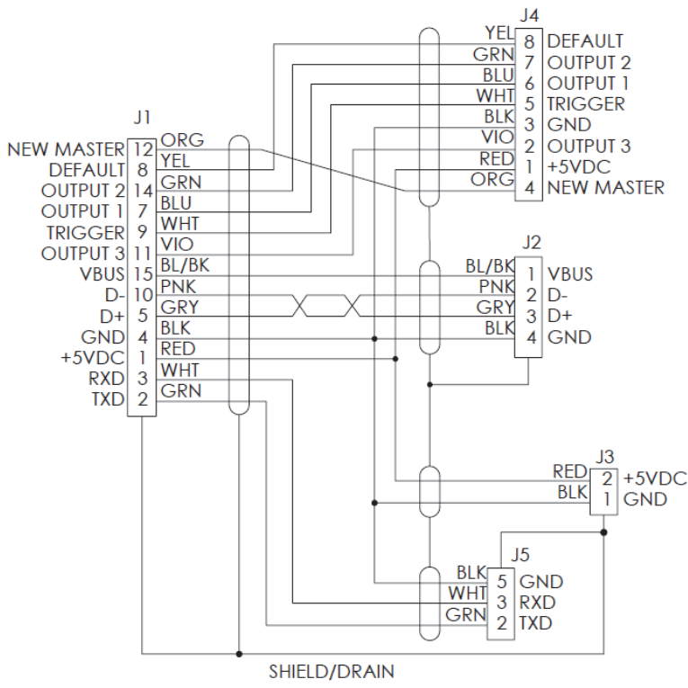
SCHEMATIC
