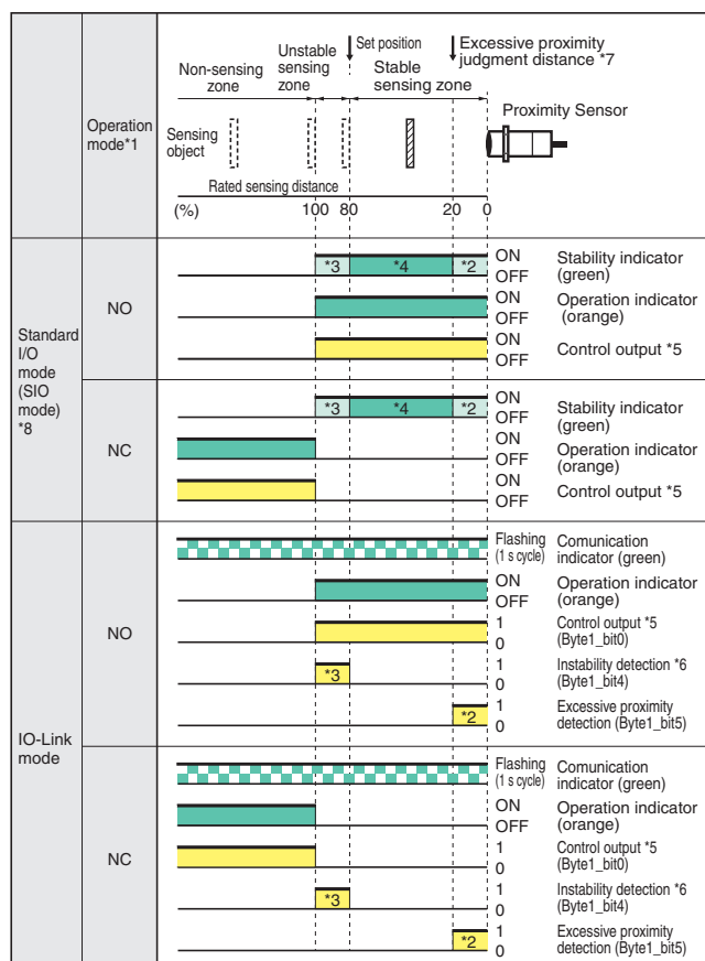
Timing Chart
