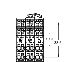
Double-contact unit Non-lighted (2NO/2NO/2NC)
