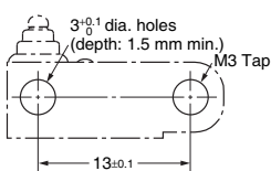
Mounting Hole Dimensions (Reference)
