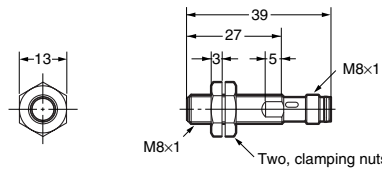
E2A-S08KS02-M5-□□
