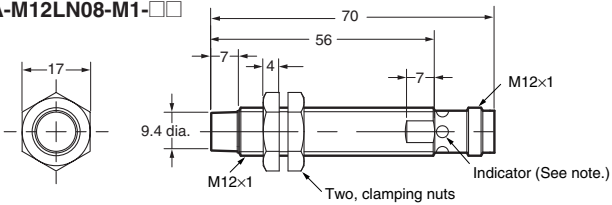
E2A-M12LN08-M1-□□
