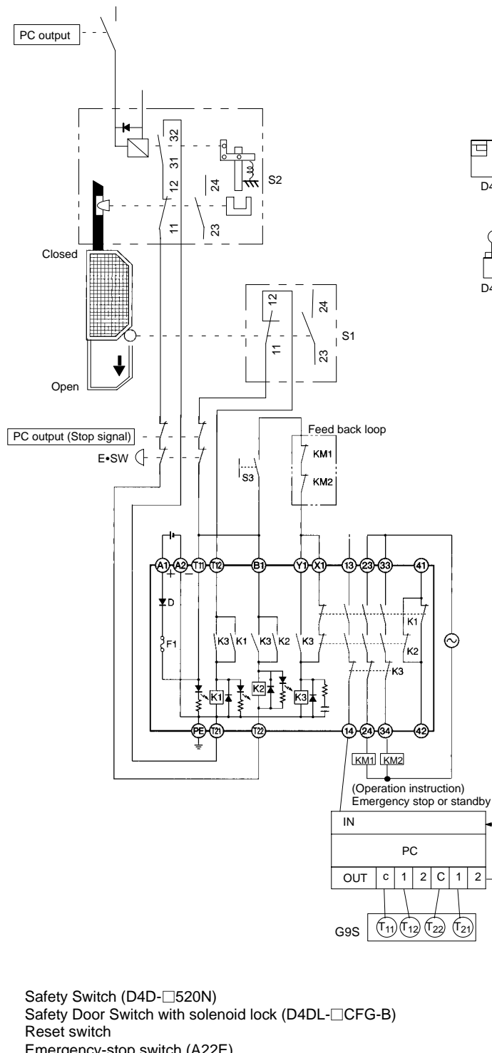
Circuit Diagram
