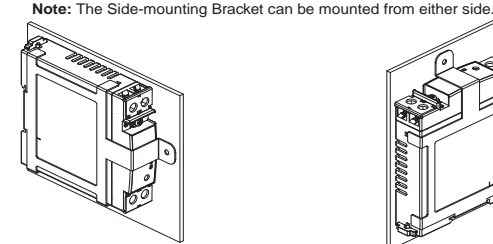
Horizontal mounting with S82Y-VS30P*
