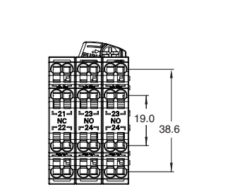
Double-contact unit Non-lighted (2NO/2NO/2NC)
