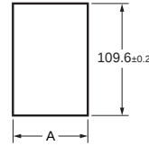
Panel Cutout (Panel thickness: 1 to 4 mm)
