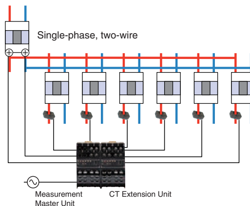
Distribution Panel for Lighting (Single-phase, Two-wire) Measurement of Six Lights
