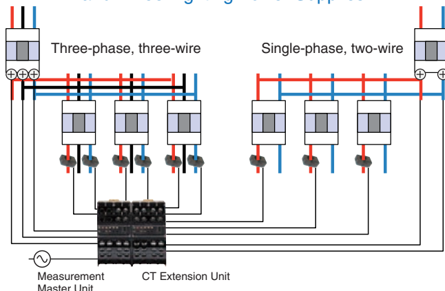
Mixed Distribution Panel for Lighting and Operation (Three-phase, Three-wire or Single-phase, Two-wire) Measurement of Three Operational Power Supplies and Three Lighting Power Supplies
