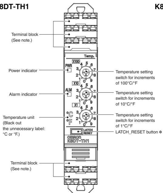
K8DT-TH1
