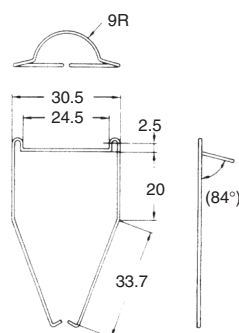
Y92H-4 for PY□ Socket
