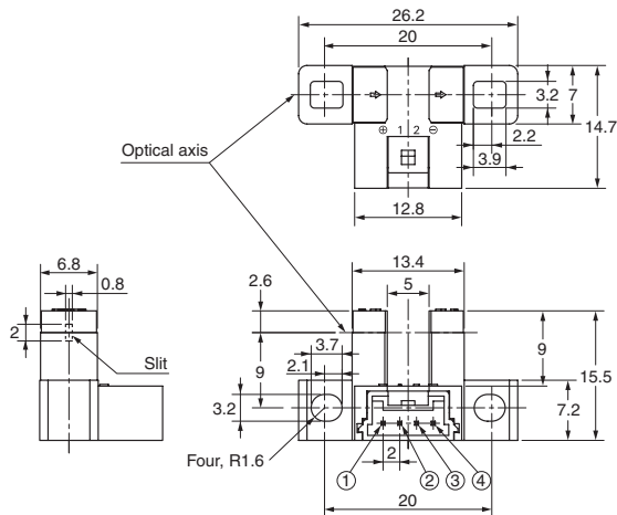
Mounting screw holes
