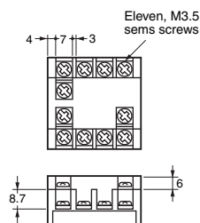
Terminal Layout/Internal Connections (Bottom View)
