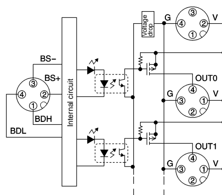
SRT2-OD0□CL-1 (PNP)
