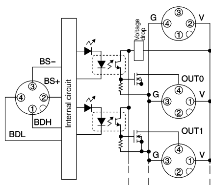
SRT2-OD0□CL (NPN)
