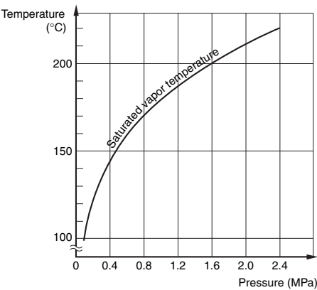
Pressure-Temperature Curve
