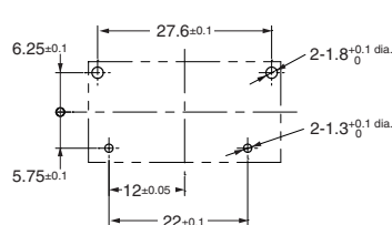
PCB Mounting Holes (BOTTOM VIEW)
