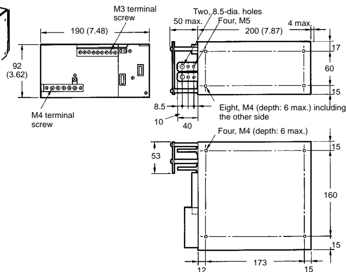
Mounting Holes Side View
