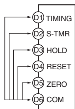
Models with Terminal Blocks <K35-1><K35-3>
