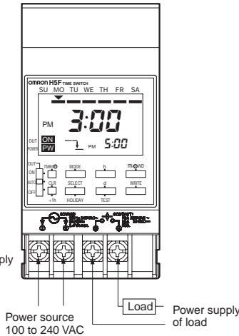
Surface Mounting/Track Mounting Models H5F-KB
