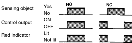
E2E2-X□C□/B□ DC 3-wire Models
