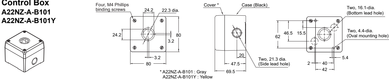
Control Box (2 holes) A22NZ-A-B102
