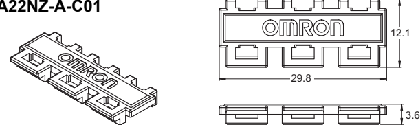
Reinforcement Plate A22NZ-A-C01
