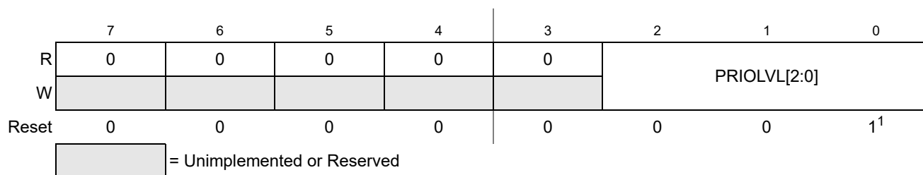
Figure 5-6. Interrupt Request Configuration Data Register 1 (INT_CFDATA1)
