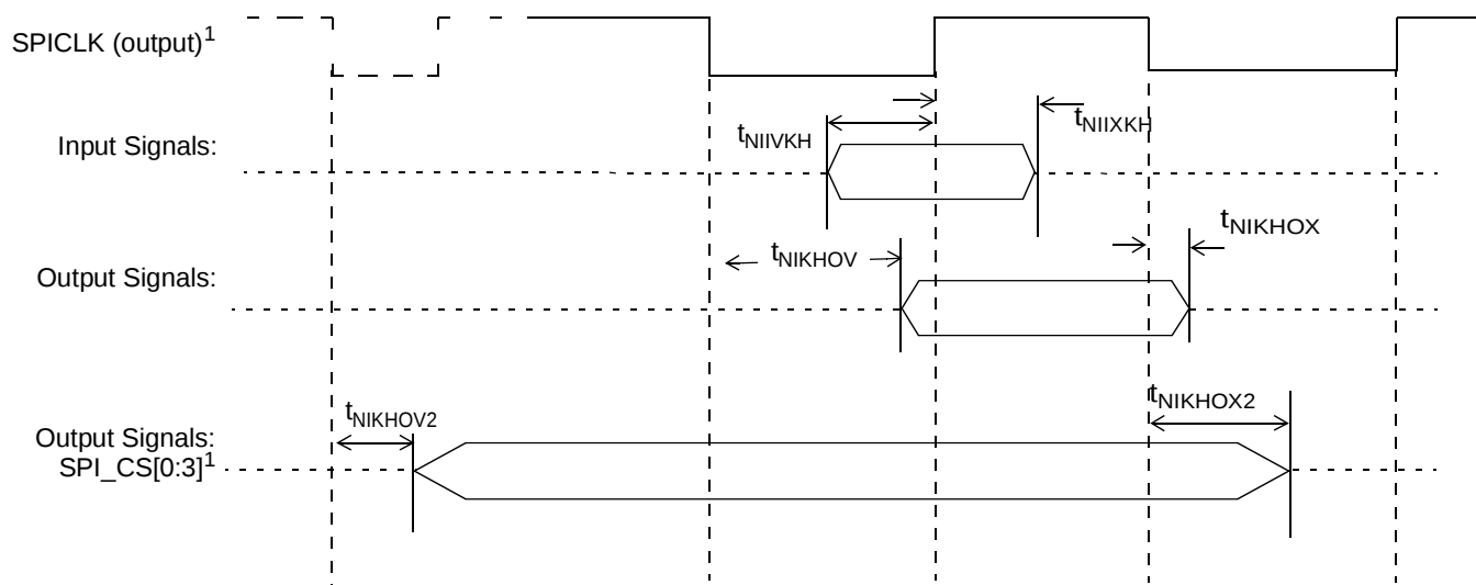
Figure 14. SPI AC Timing in Master Mode (Internal Clock) Diagram
