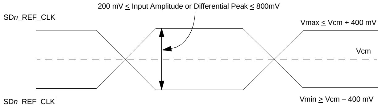
Figure 48. Differential Reference Clock Input DC Requirements (External AC-Coupled)
