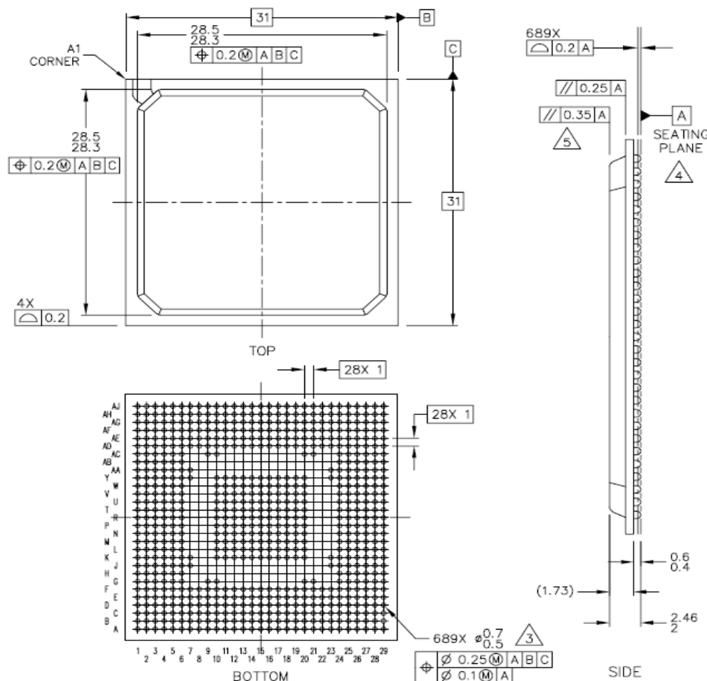
Figure 54. P1020 Package
