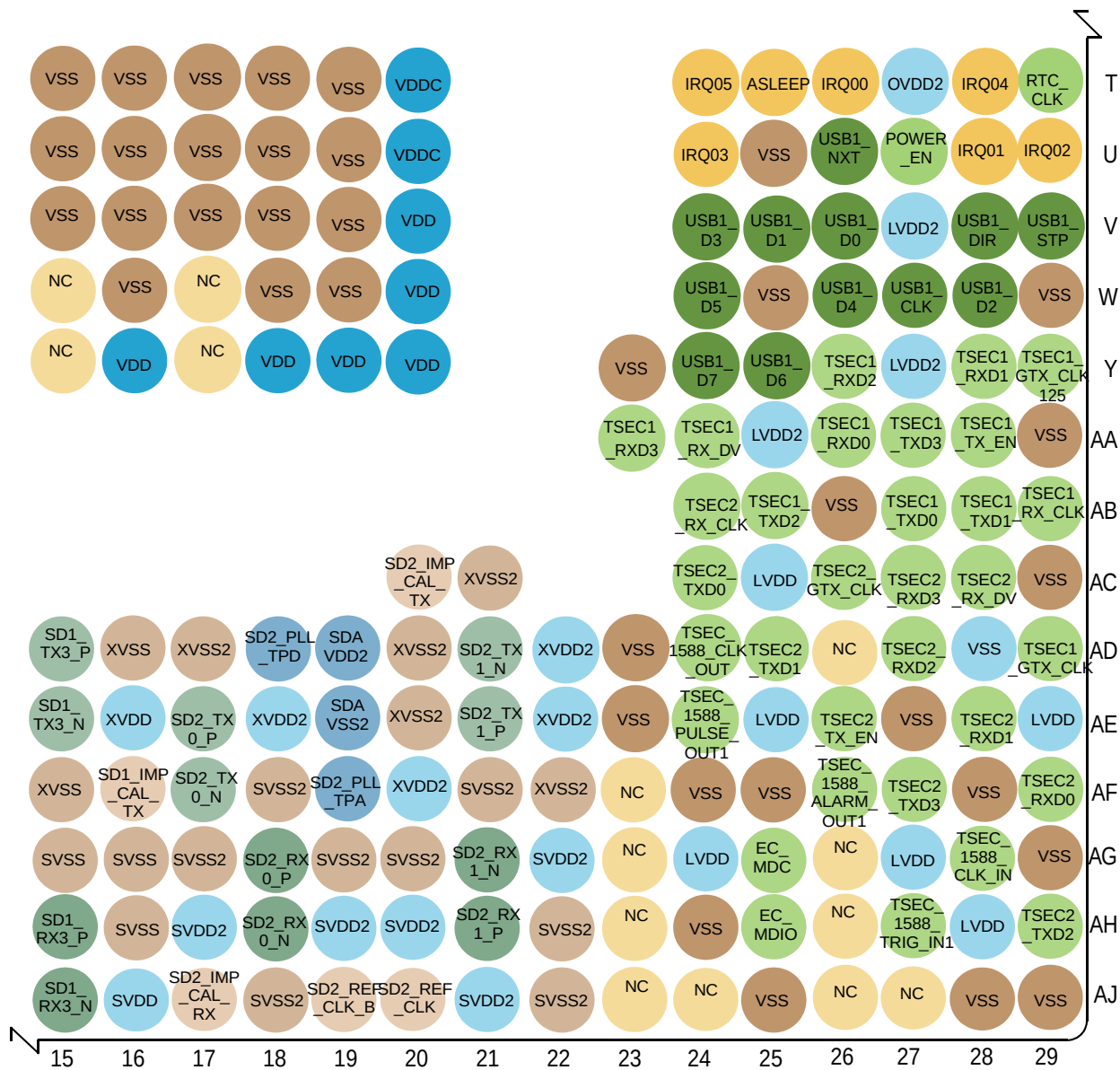
DETAIL D
