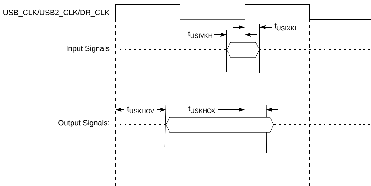
Figure 27. USB signals
