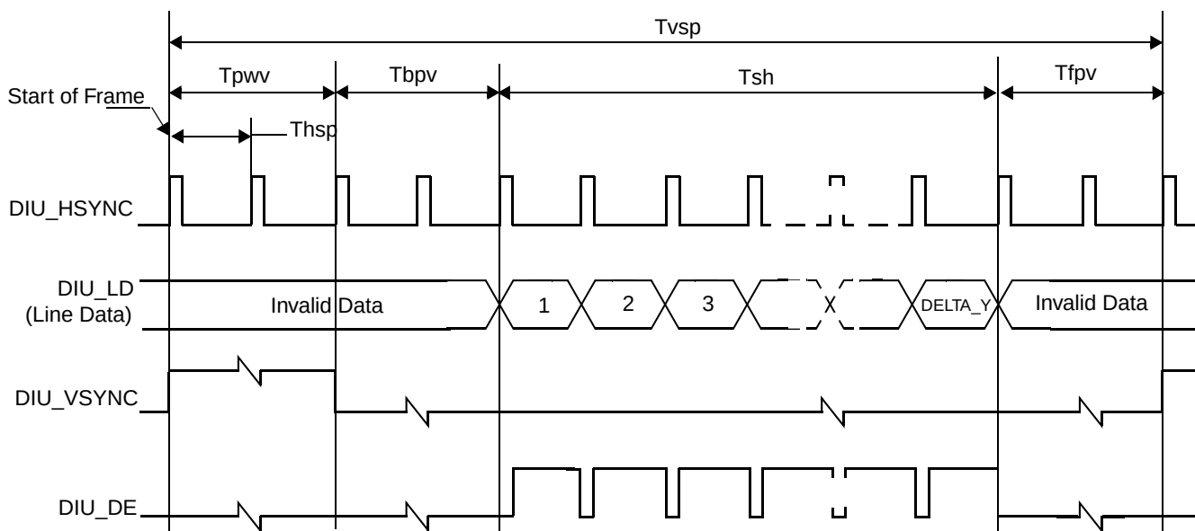
Figure 34. TFT DIU/LCD interface timing diagram—vertical sync pulse
