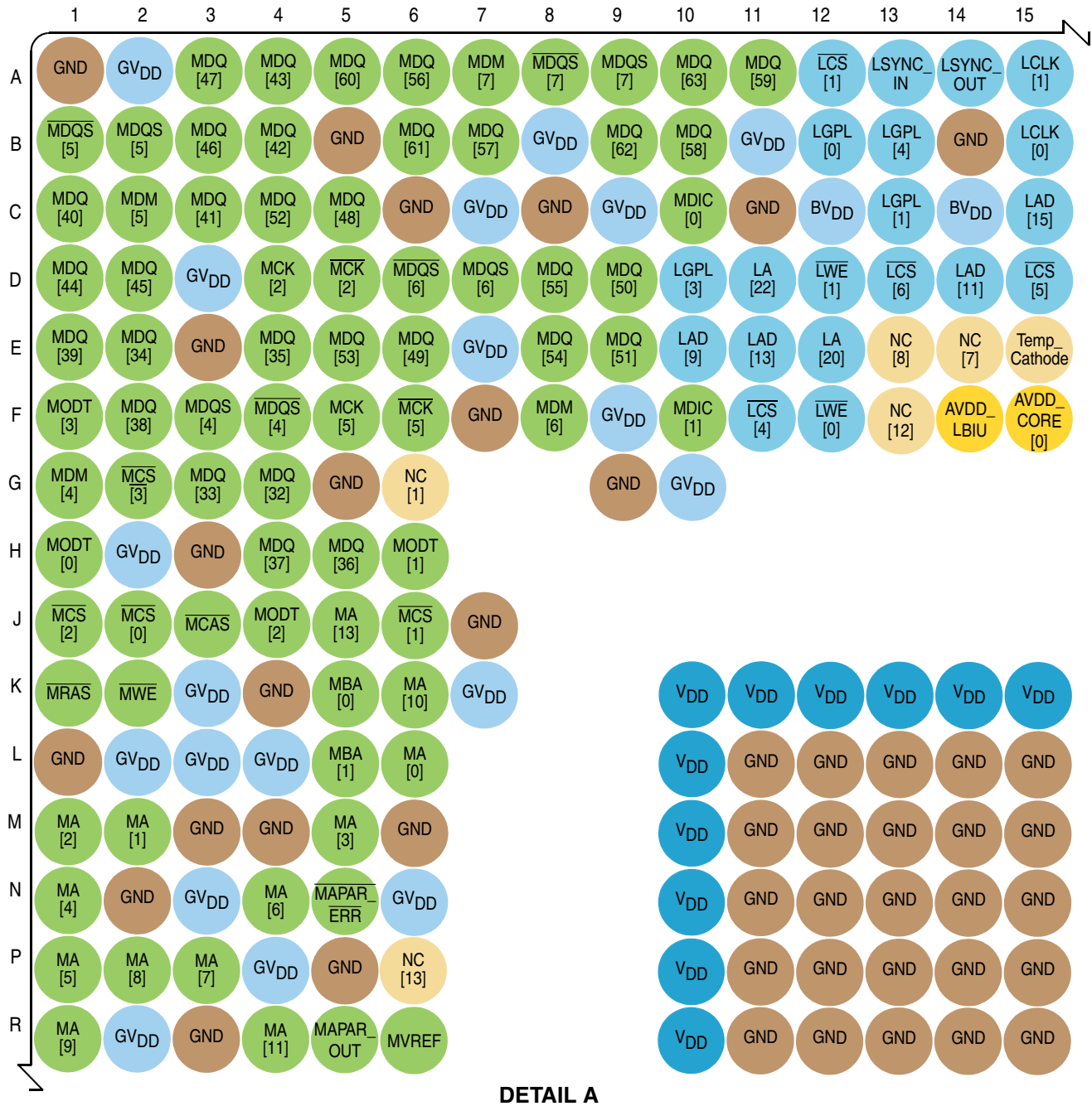
Figure 3. P2020 Ball Map—Detail A
