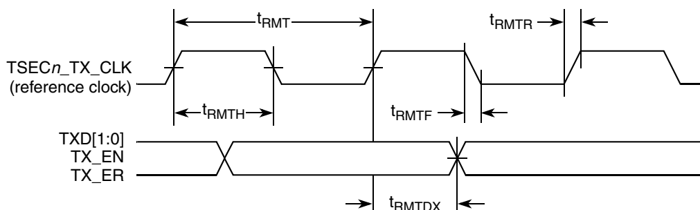
Figure 24. RMII Transmit AC Timing Diagram
