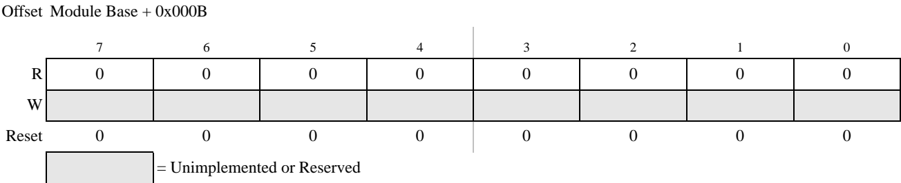
Figure 18-17. Flash Reserved1 Register (FRSV1)
