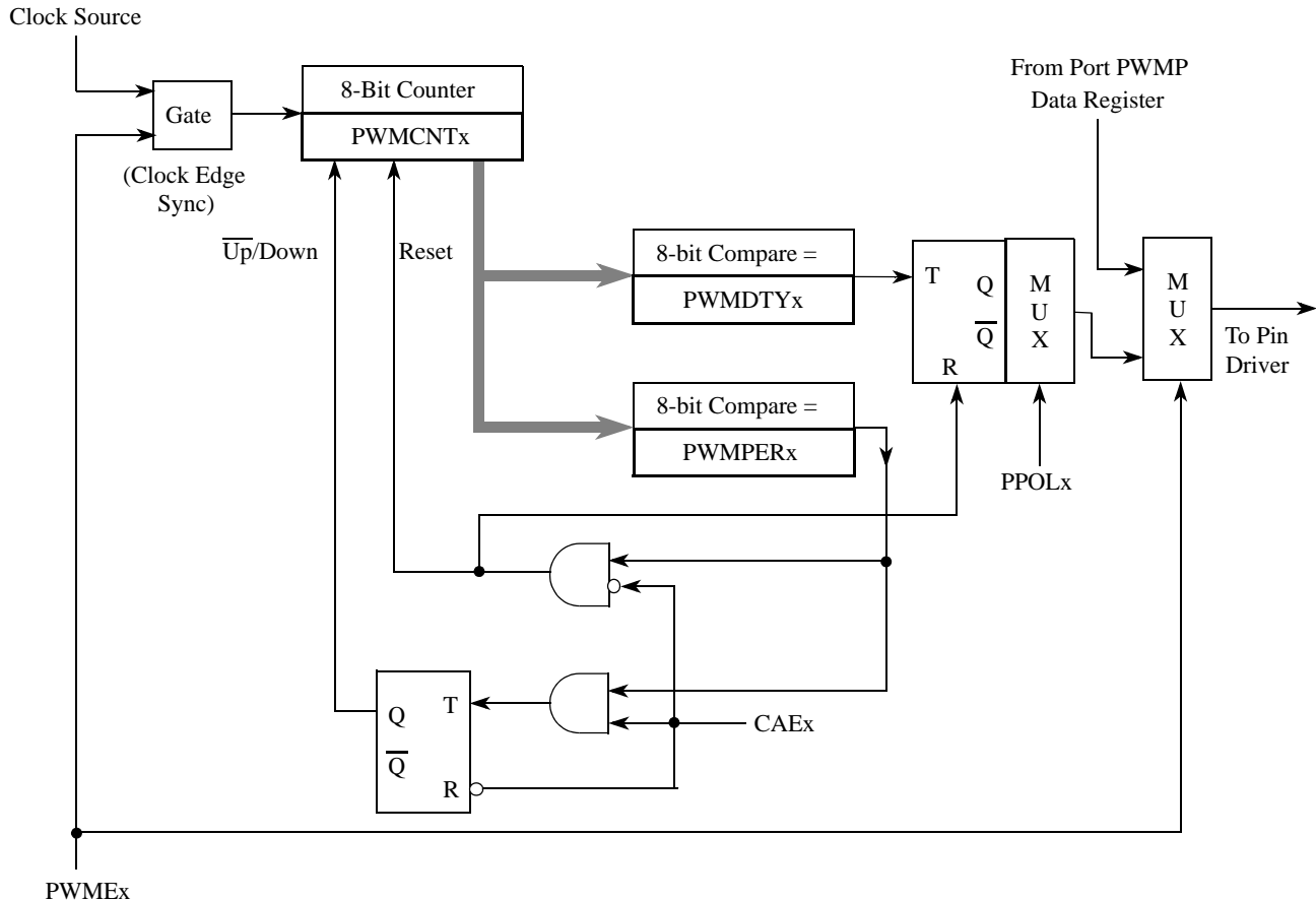
Figure 13-16. PWM Timer Channel Block Diagram
