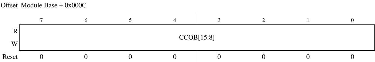
Figure 18-18. Flash Common Command Object 0 High Register (FCCOB0HI)
