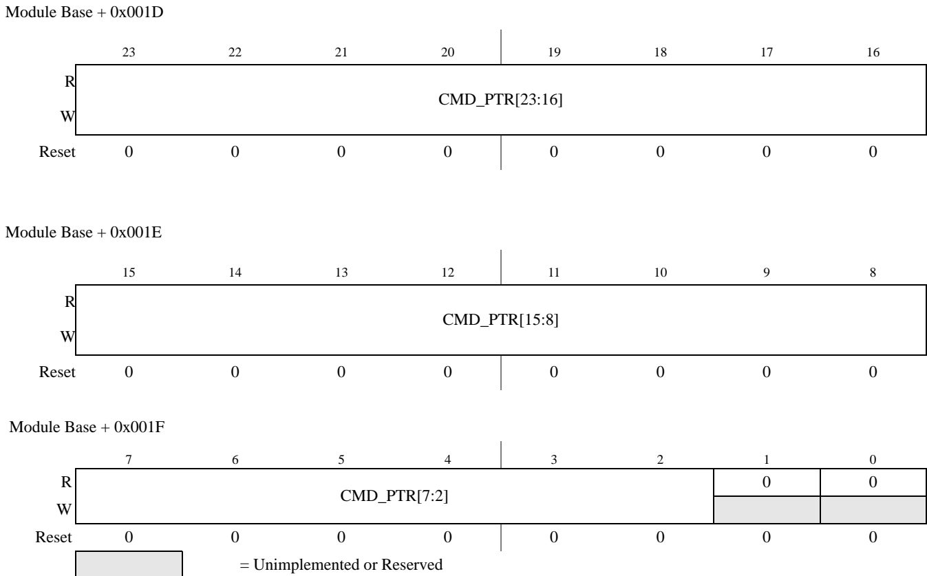
Figure 9-23. ADC Command Base Pointer Registers (ADCCBP_0, ADCCBP_1, ADCCBP_2))
