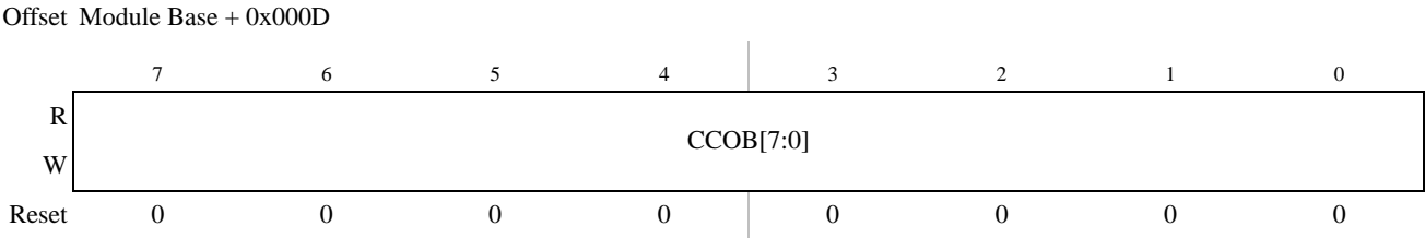
Figure 18-19. Flash Common Command Object 0 Low Register (FCCOB0LO)
