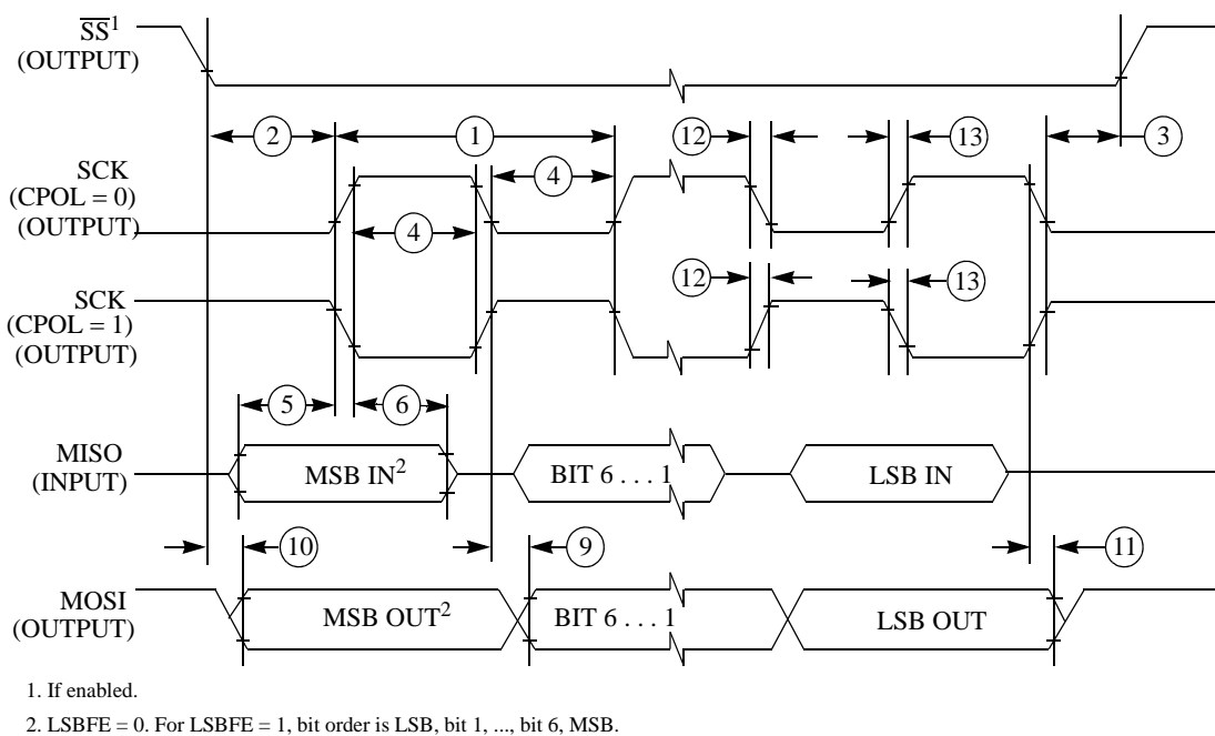
Figure A-7. SPI Master Timing (CPHA=0)
